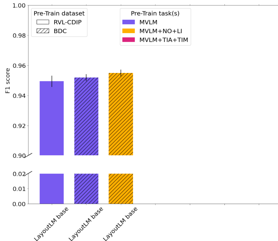
Figure 12: Specific pre-training tasks improve performance on document understanding tasks
