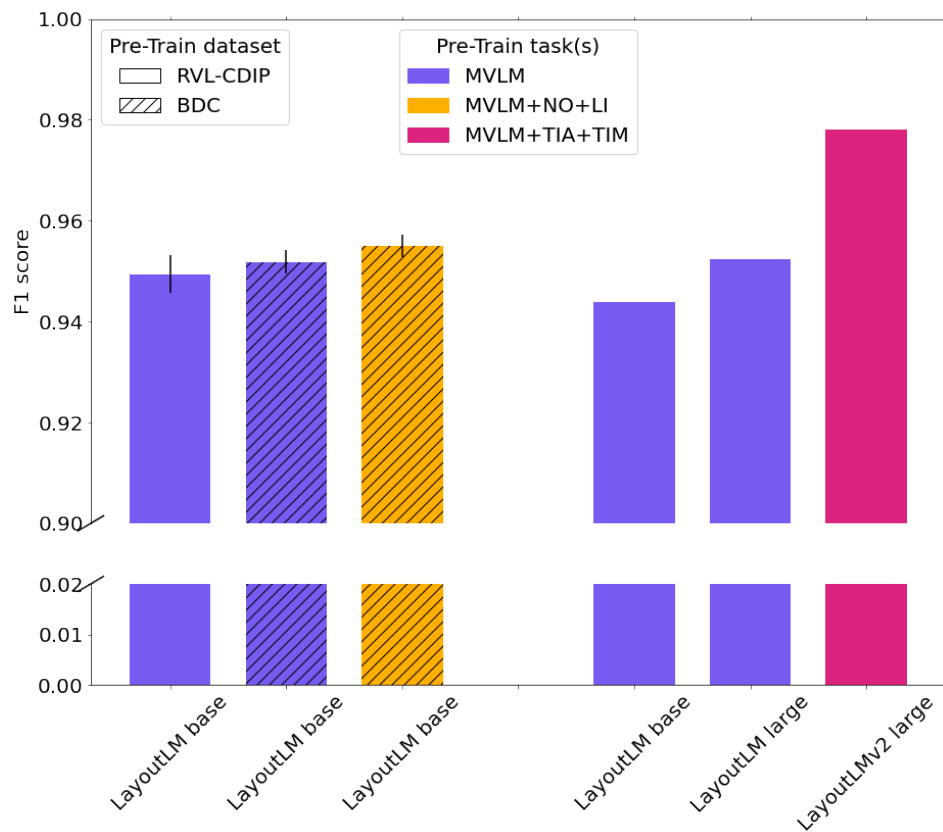
Figure 13: Up to the performance of a model 3\times larger
