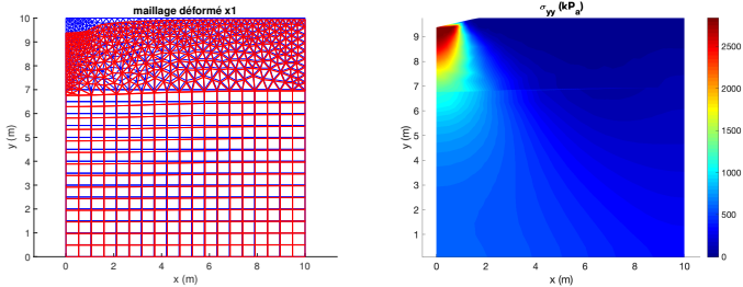
FIGURE — Example of results coming from FEM computation.
