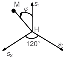
FIGURE — graphical illustration of the Lode's angle
